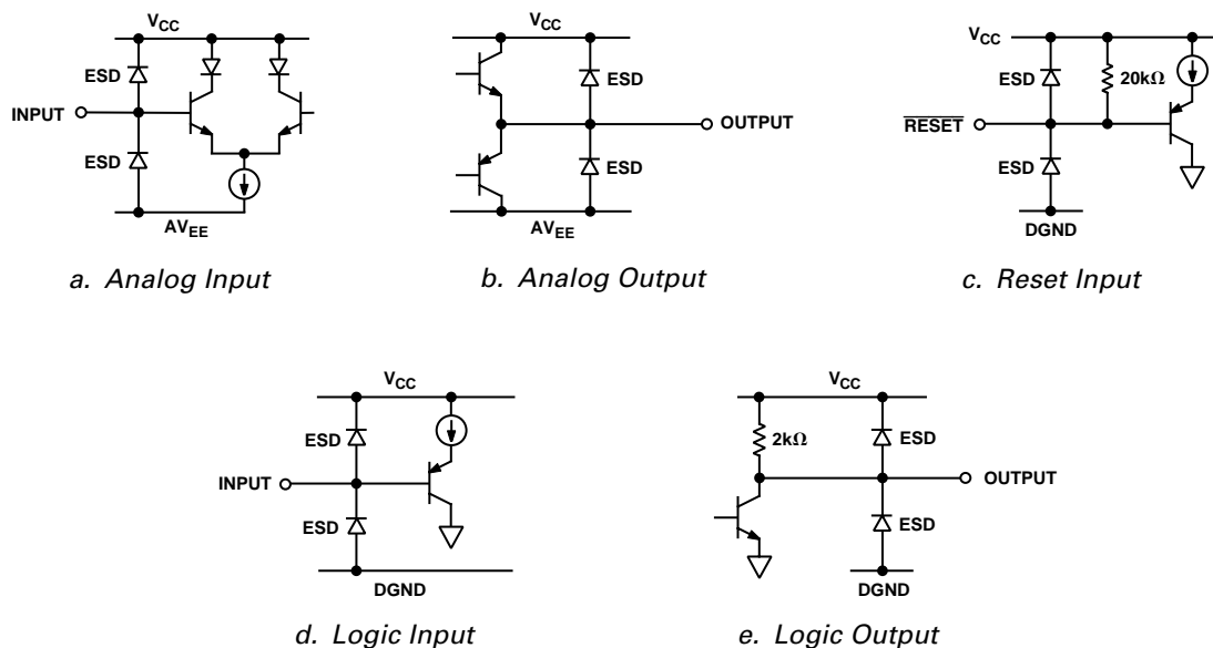
Figure 5. I/O Schematics
